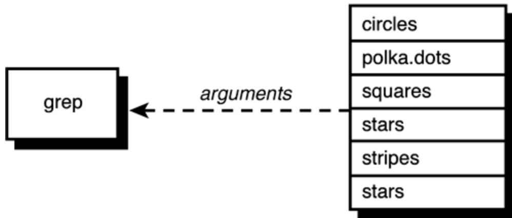
Figure 4.1. grep * stars .
