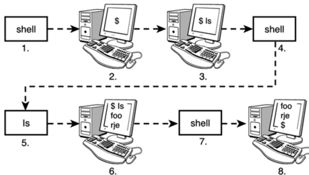
Figure 3.6. Command cycle.
