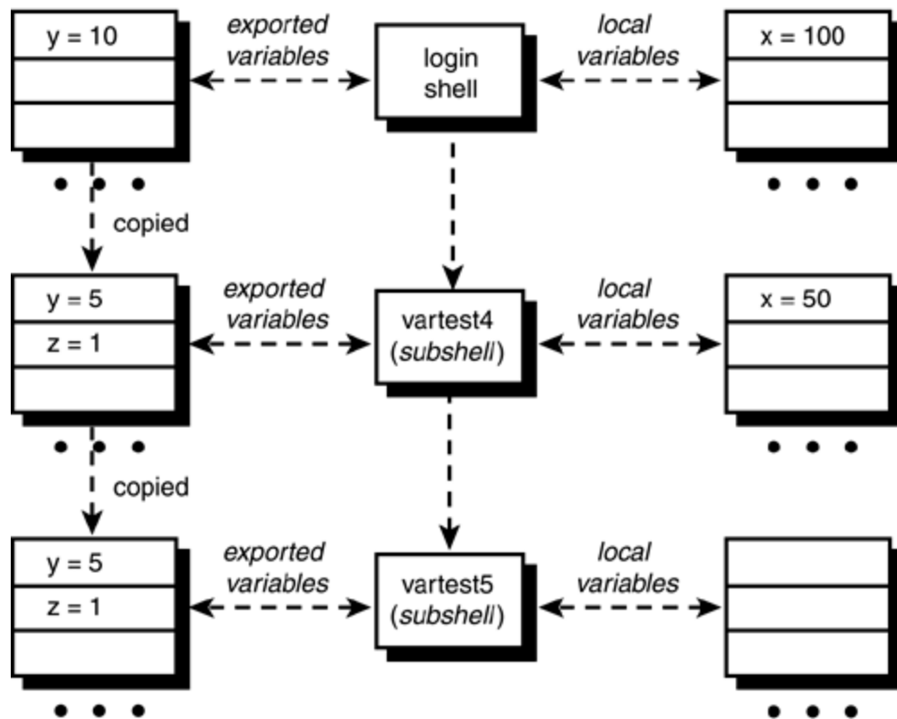
Figure 11.6. Subshell execution.
