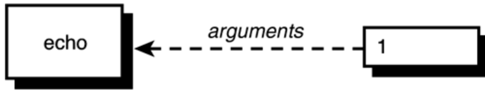
Figure 5.1. echo $count .
