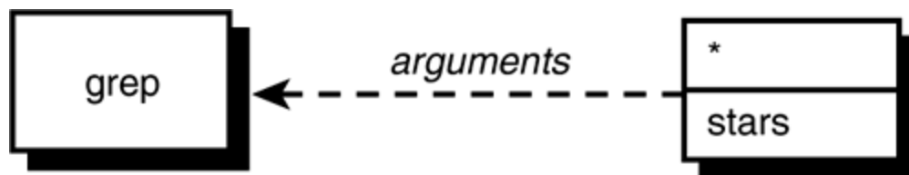
Figure 4.2. grep '*' stars .
