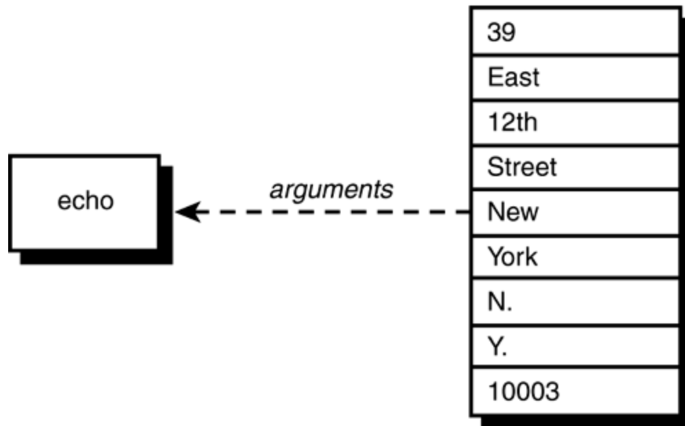
Figure 6.5. echo $address .
