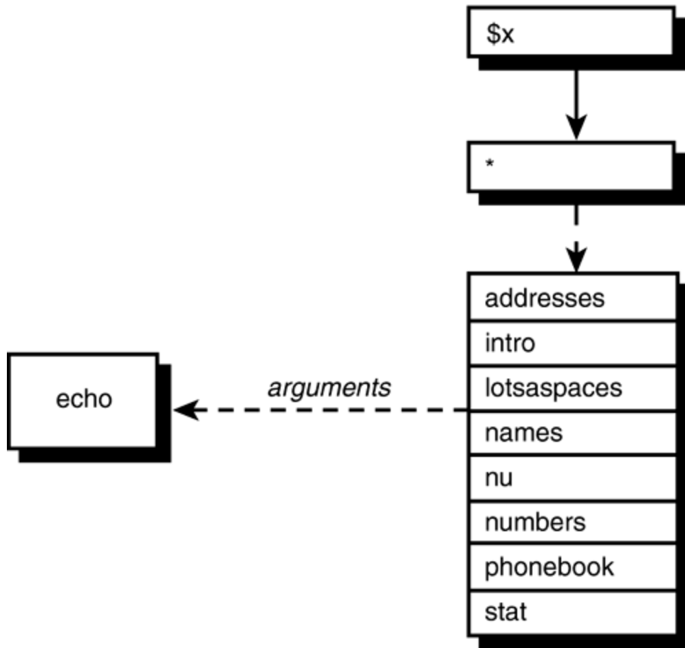
Figure 5.3. echo $x .
