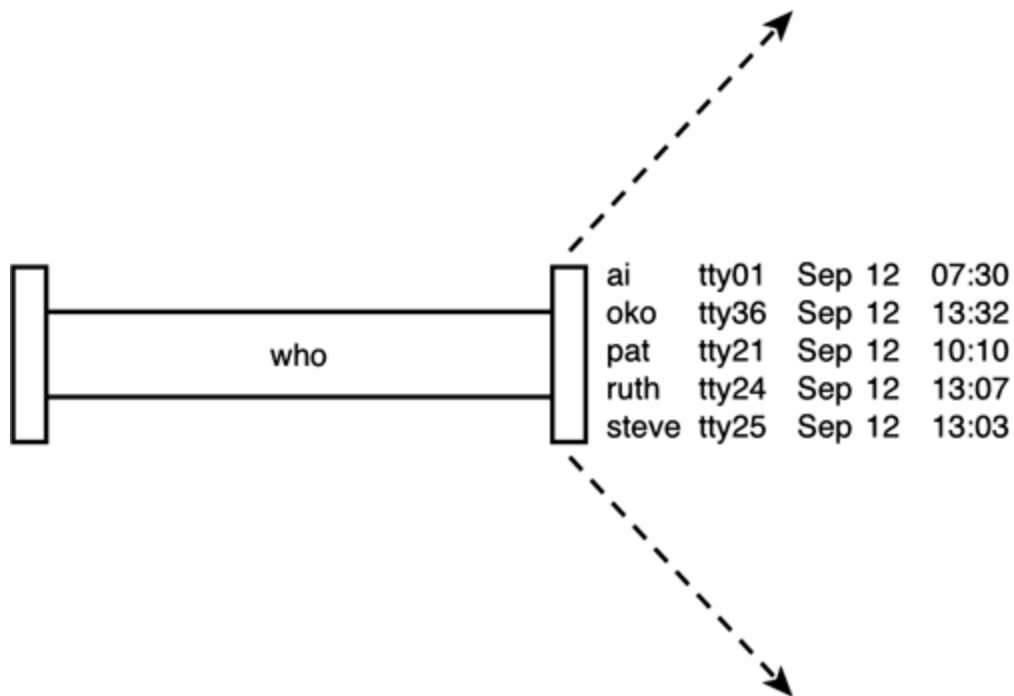
Figure 2.10. who command.
